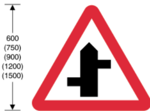
507.1 Staggered junction ahead
