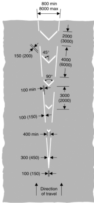
1041 Part of the carriageway where vehicular traffic passes in the same direction on both sides of the marking, and should not enter the area covered by the marking unless it is seen by the driver to be safe to do so
