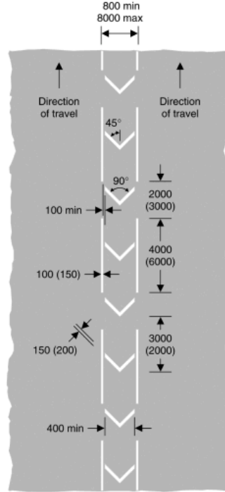
1041.1 Length of road along which vehicular traffic travels in the same direction on both sides of the marking, and should not enter the area covered by the marking unless it is seen by the driver to be safe to do so
