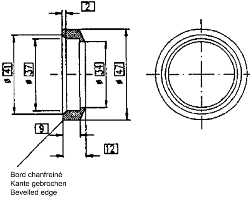
Fig. I.14 Coupling Head — Main Reservoir Pipe U.K.
