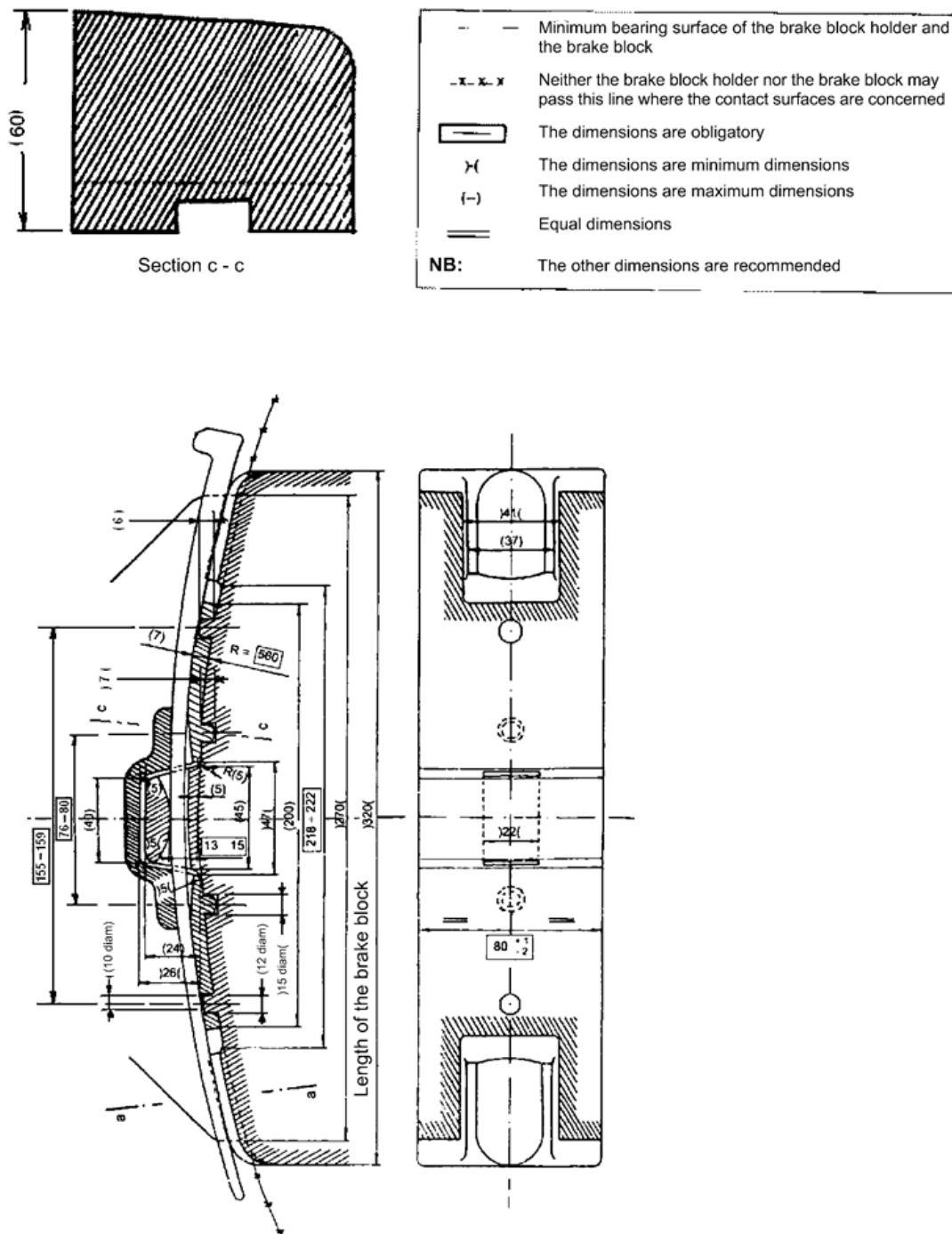
Fig I.10.3.4 All other dimensions as Fig I.10.3.2 U.K.
