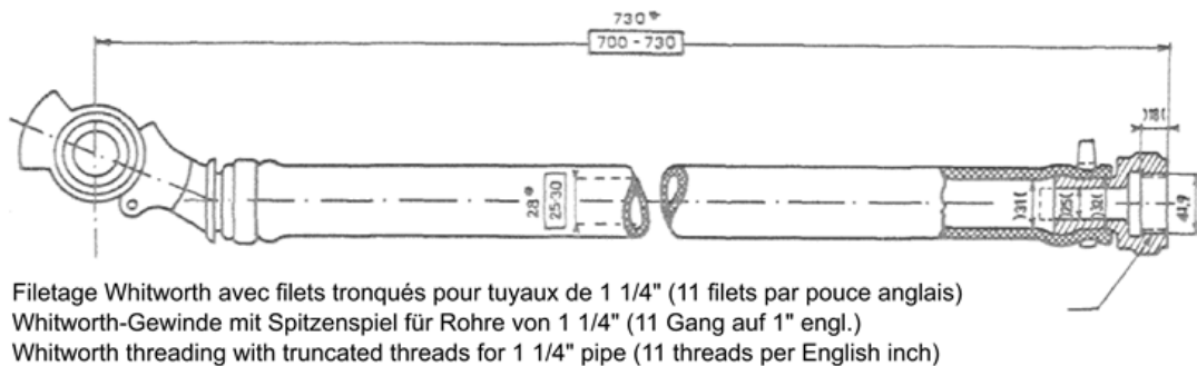
Fig. I.11 Pneumatic half coupling — Main Reservoir Pipe U.K.
