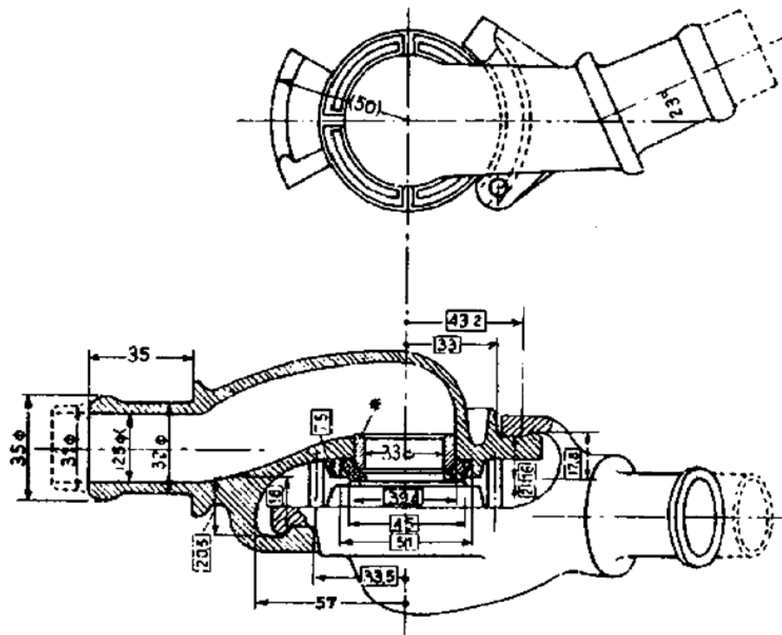
Fig. I.13 Seal — Single piece coupling head U.K.
