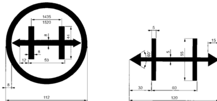
B.31. Marking on bogies with variable-gauge wheelsets (1 435 mm/1 520 mm) U.K. Fig B50
