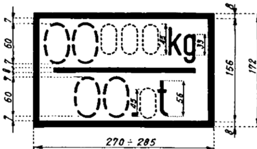
Fig. B2 Marking for the tare weight and braked weight of wagons fitted with handbrakes. U.K.
