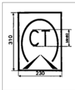
Fig. B9 for wagons accepted through the Channel Tunnel U.K.
