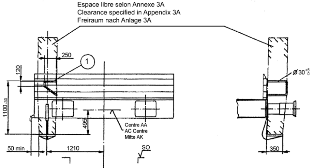
Fig. A7 Clearance to be provided at wagon extremities above the draw hook U.K.
