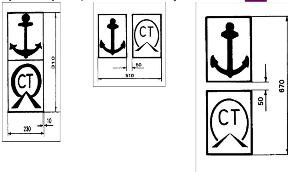
Fig. B10 for wagons accepted on train-ferries and through the Channel Tunnel U.K.
