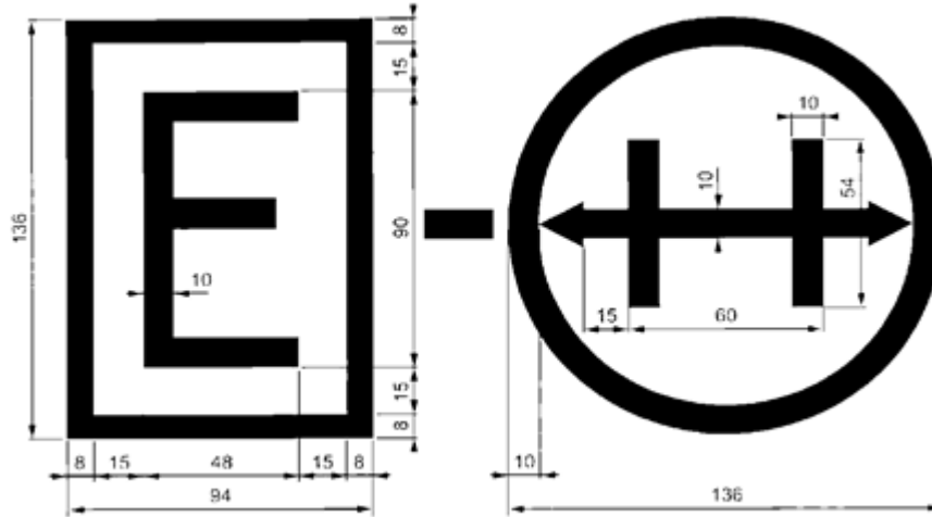
B.31. Marking on bogies with variable-gauge wheelsets (1 435 mm/1 520 mm) U.K. Fig B50
