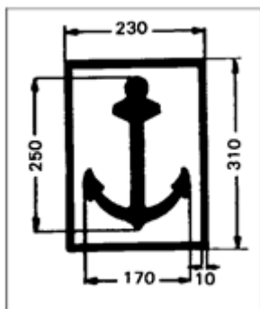
Fig. B9 for wagons accepted through the Channel Tunnel U.K.
