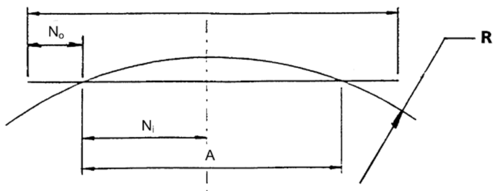
Fig.U5 Kinematic gauge WM-1 U.K.
