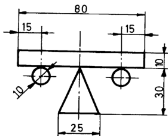
Fig. B20 Lifting with or without running gear or rerailing by only one extremity or close to the extremity. U.K.
