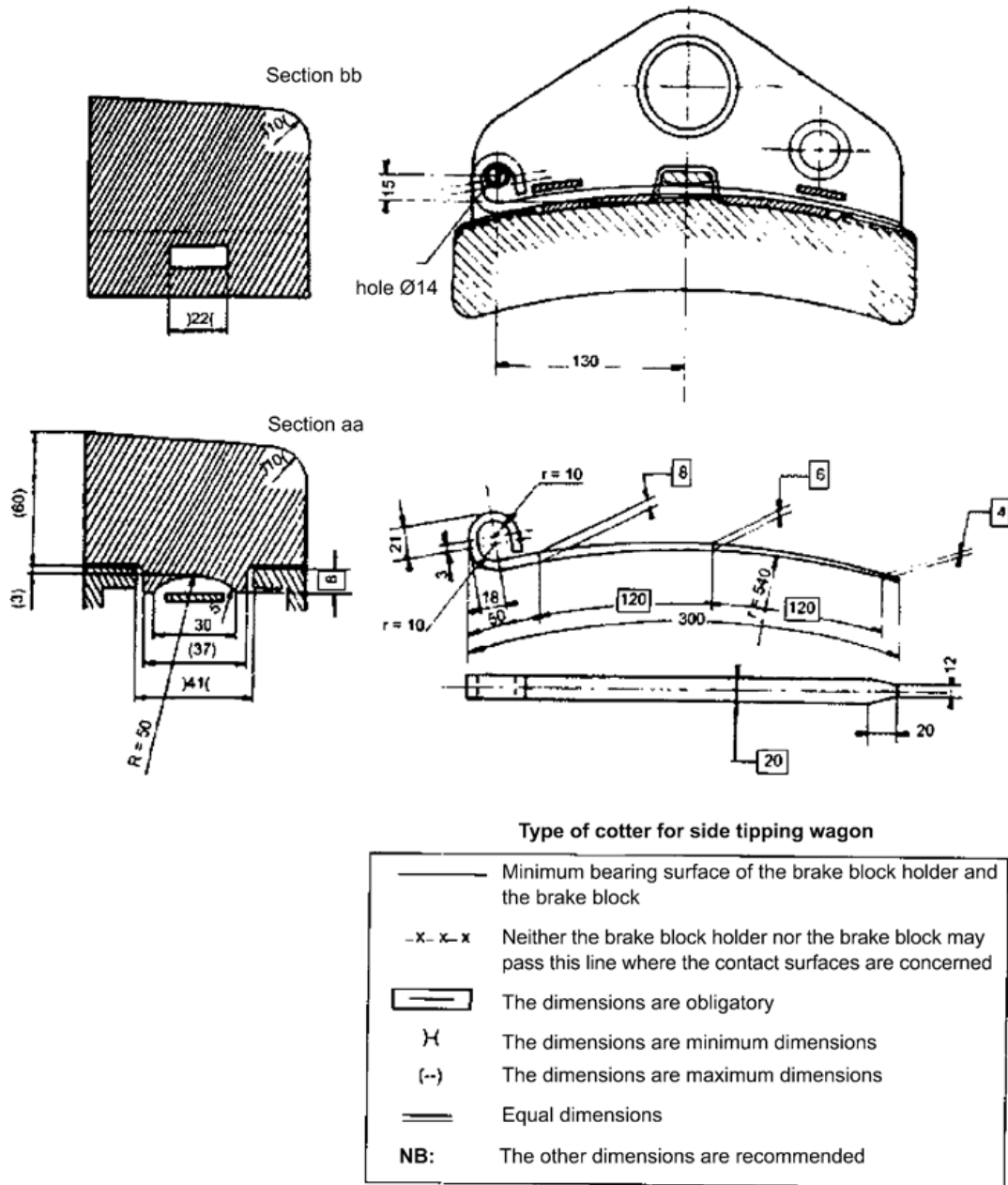
Fig I.10.3.3 All other dimensions as Fig I.10.3.1 U.K.
