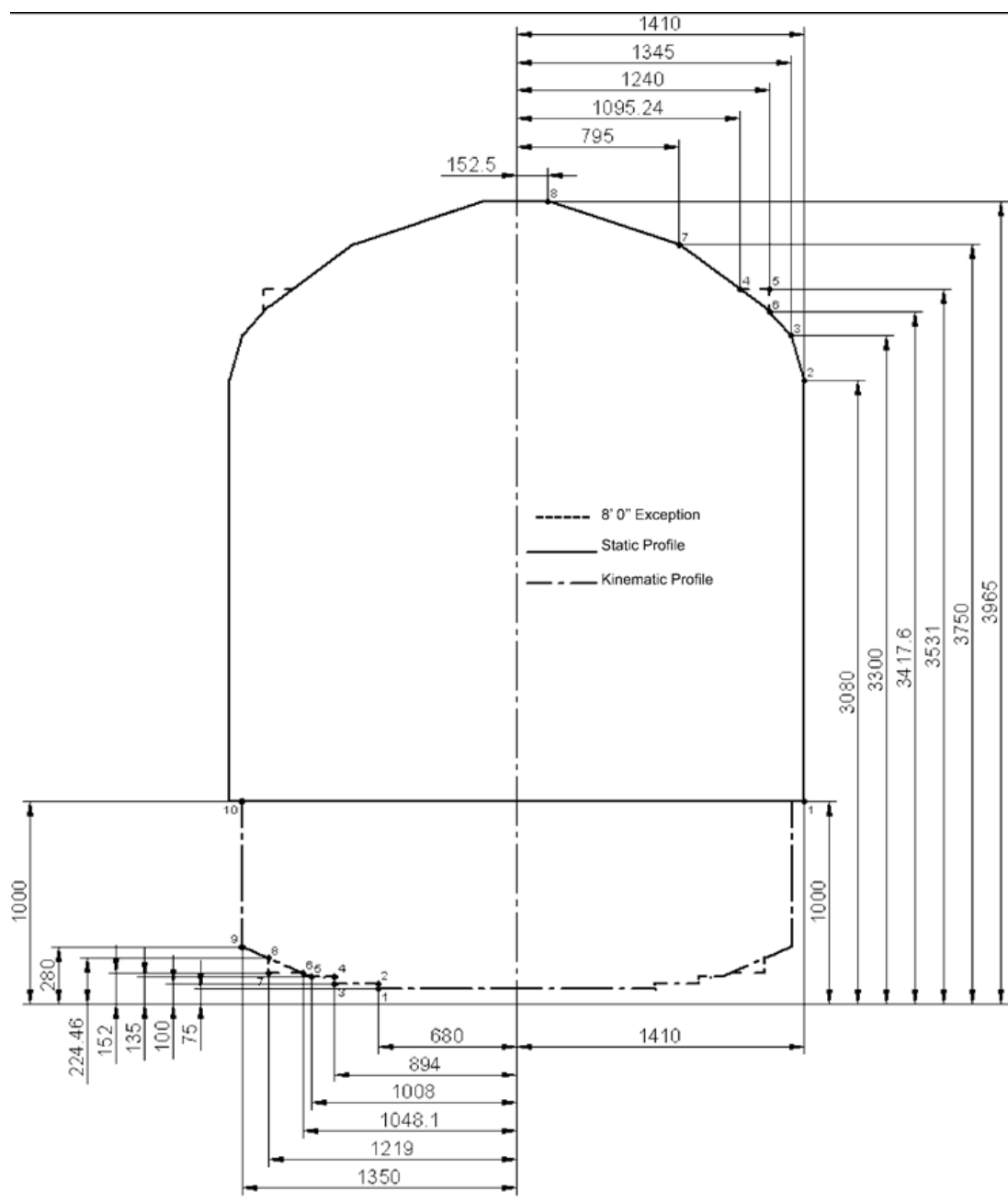
Fig. U6 Lower parts for kinematic gauge WM-02, 1, 0 U.K.
