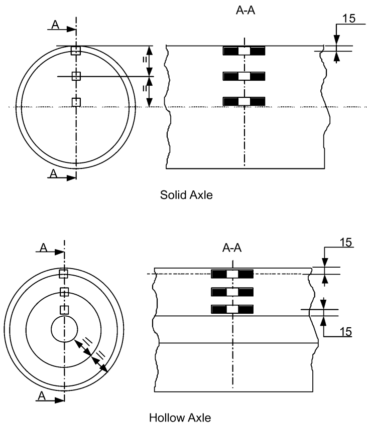
Hollow Axle
