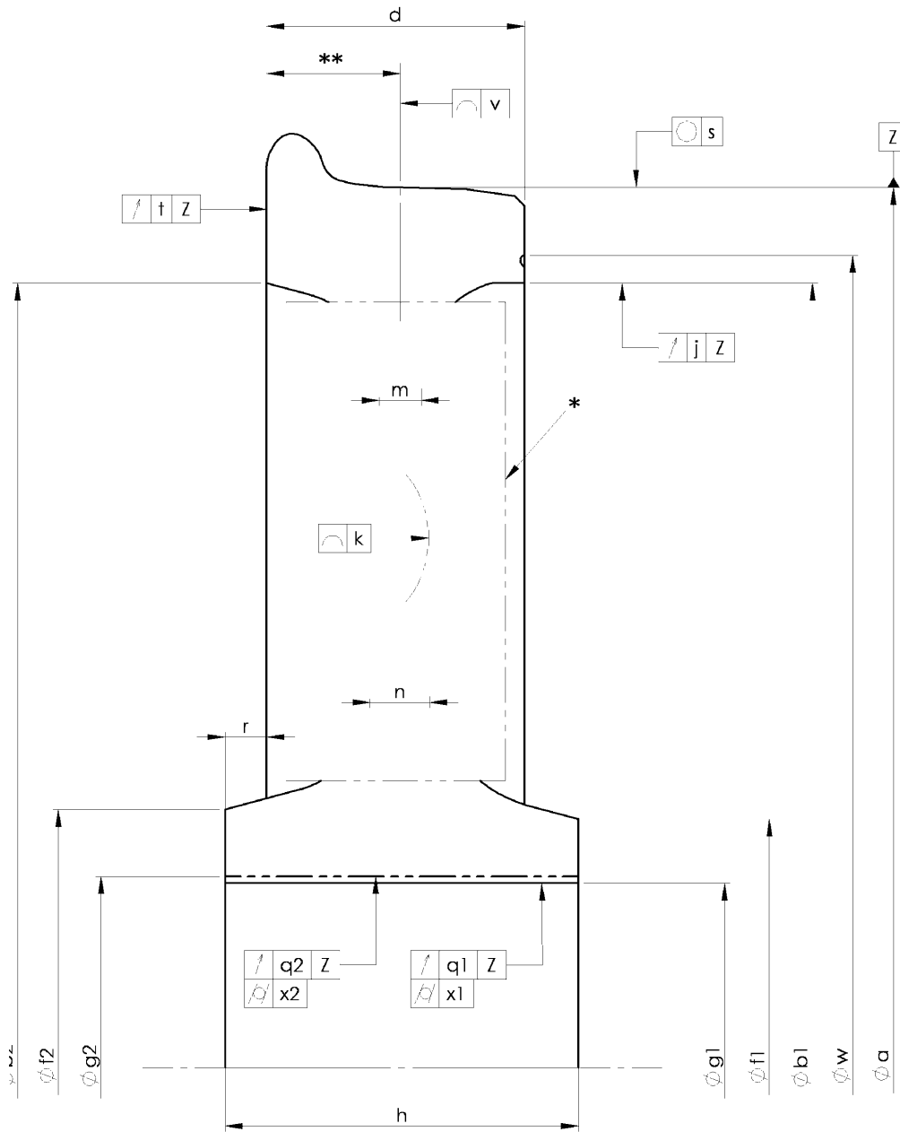
Figure L4 Symbols
