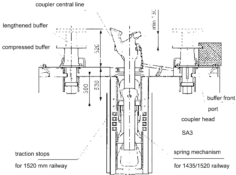
Coupler Version D
