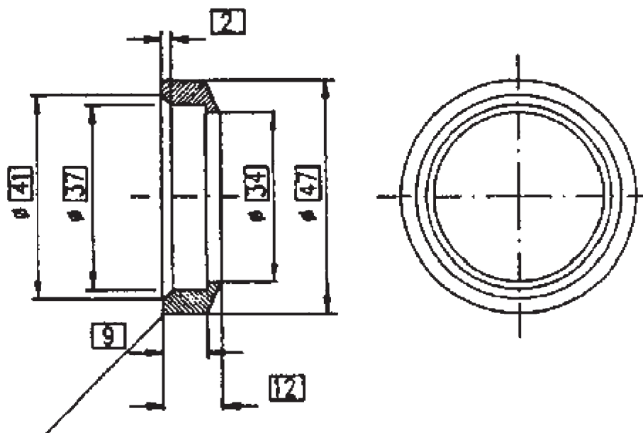
Fig. I.13 Seal — Single piece coupling head
