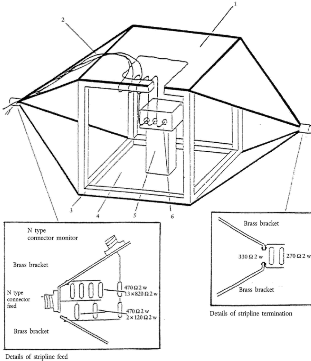
Figure 1 800 mm stripline testing U.K.
