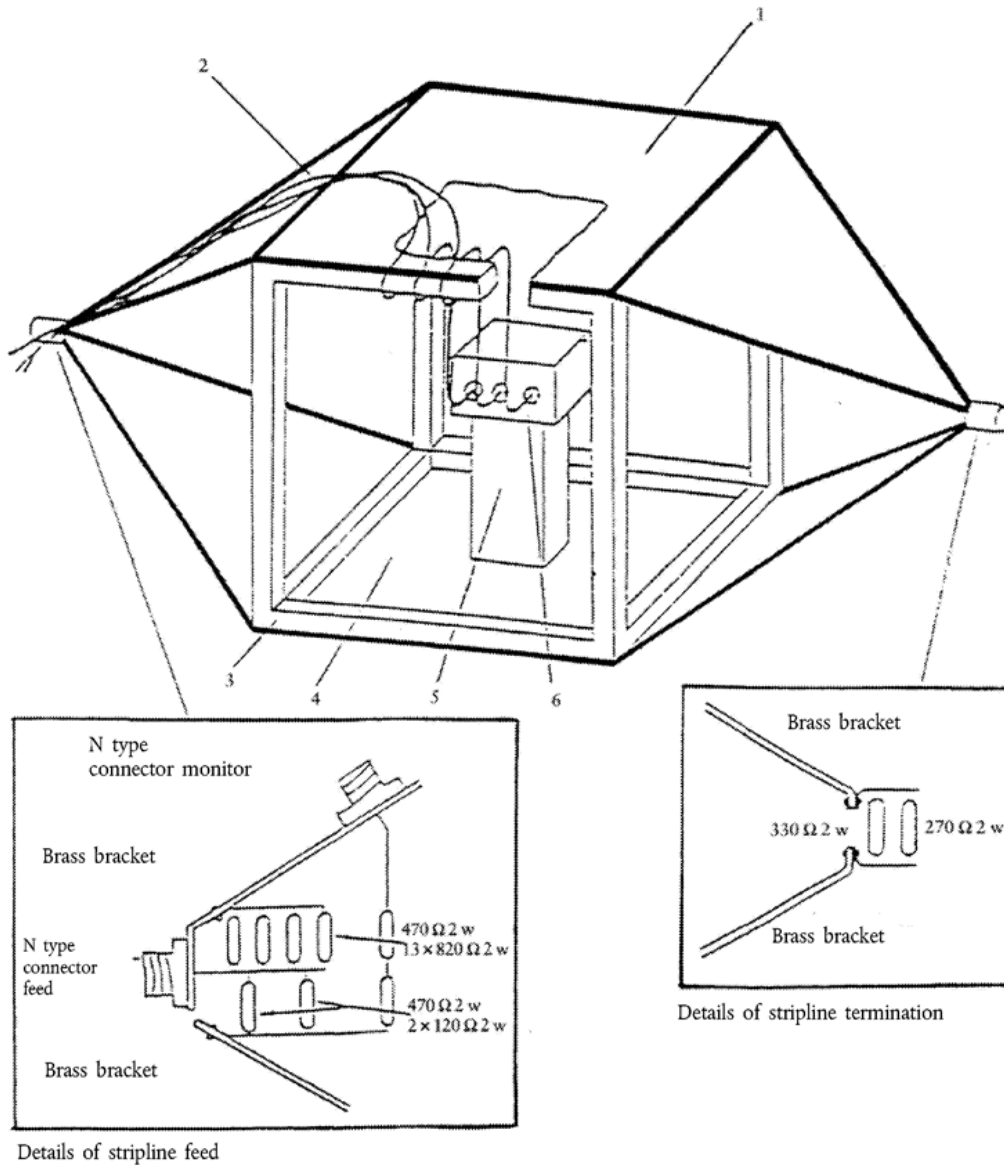
Figure 1 800 mm stripline testing
