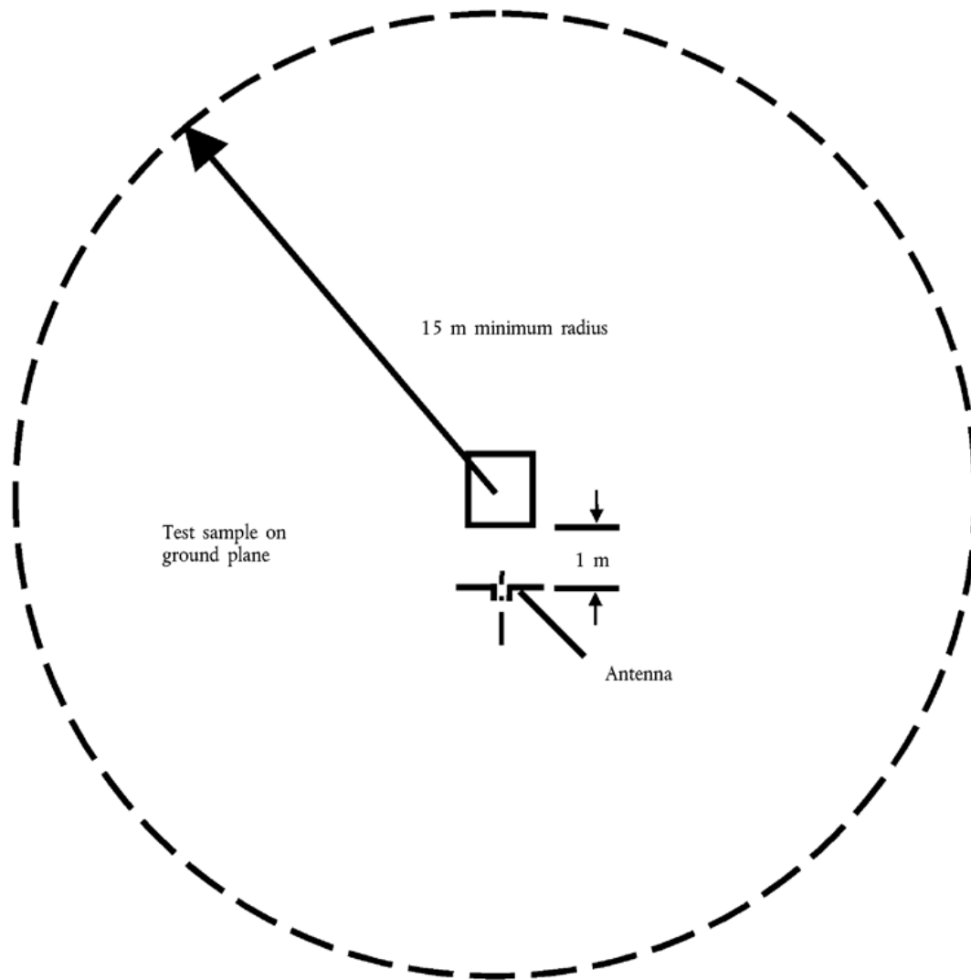
Figure 1 Open-area test site: Electrical/electronic subassembly test area boundary Level, clear area free from electromagnetic reflecting surfaces
