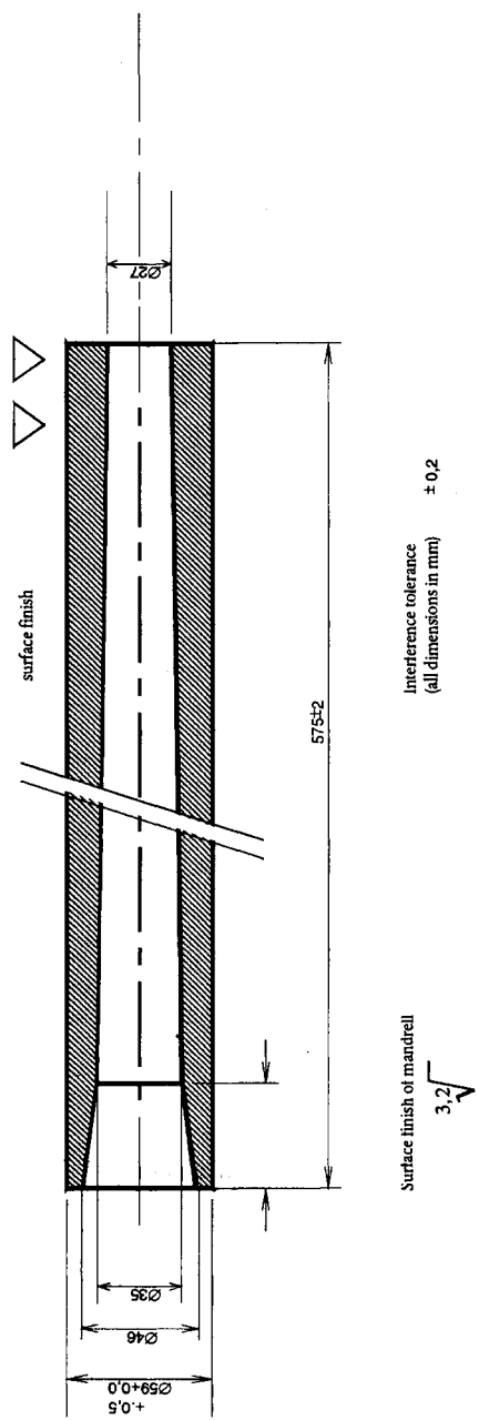
Figure 3 Stopping device (polyurethane tube)
