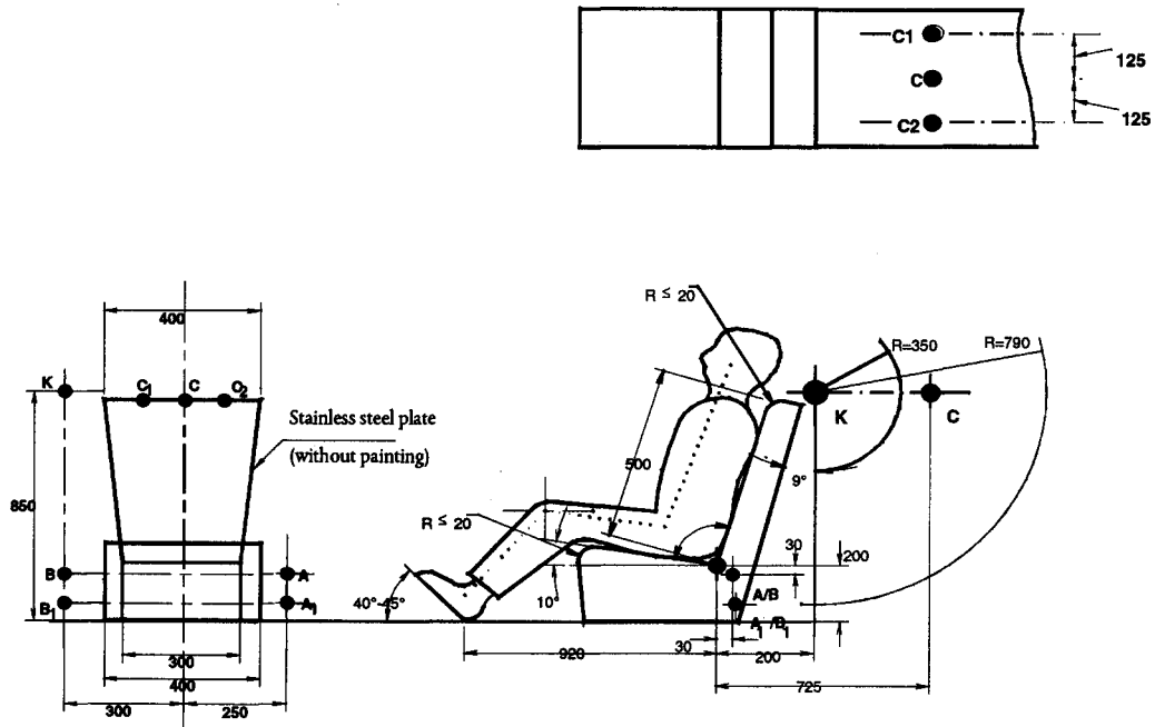
Figure 1 Trolley, seat, anchorage
