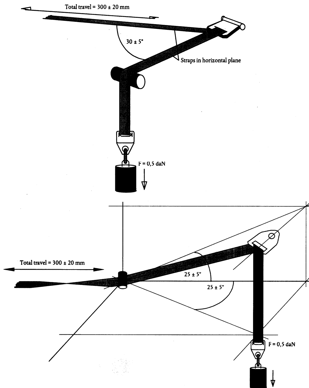
Figure 2 Type 2 test
