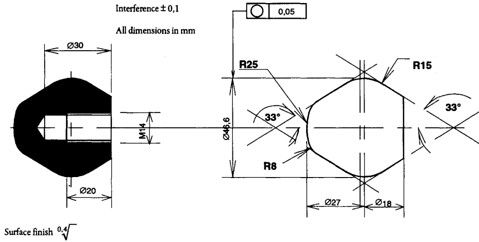
Figure 4 Stopping device (olive-shaped knob)
