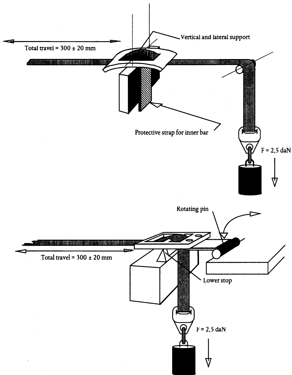
Figure 1 Type 1 test
