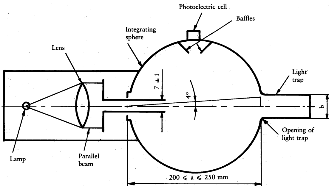
Figure 5 Hazameter
