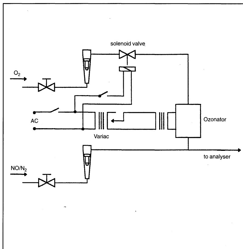
Schematic of NO 2 converter efficiency device
