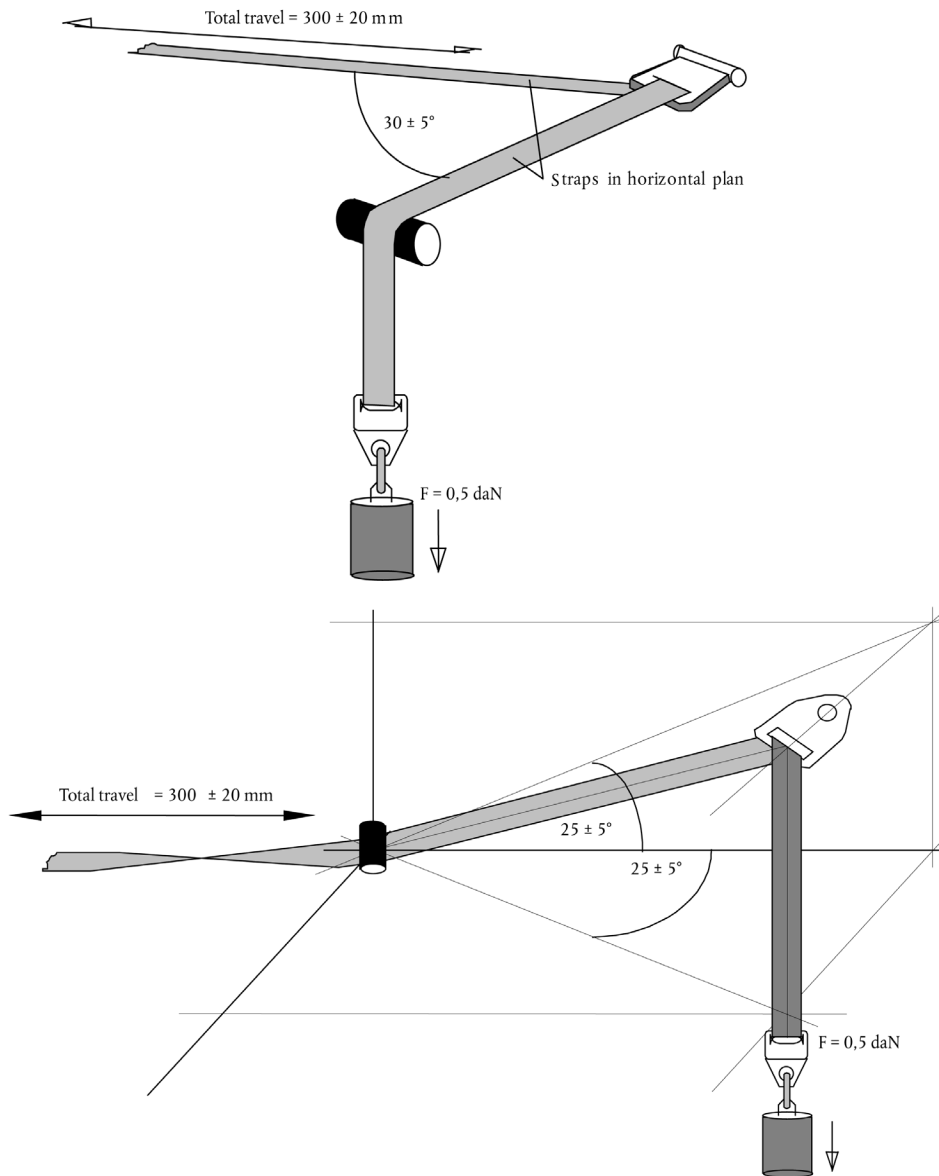
Figure 2 Type 2 test
