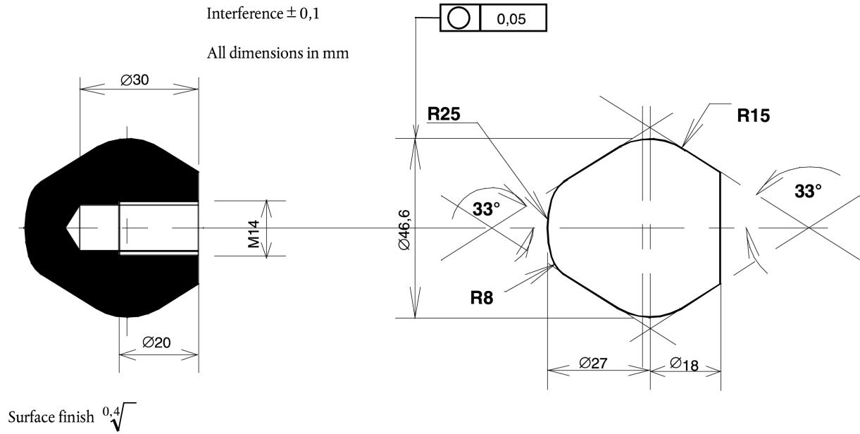
Figure 4 Stopping device (olive-shaped knob)
