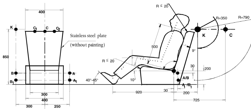
Figure 1 Trolley, seat, anchorage
