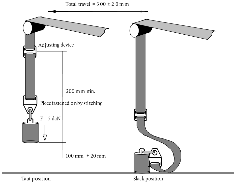
Figure 3 Type 3 test and microslip test
