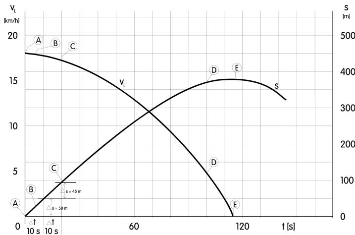
Figure 1 Stopping manoeuvre
