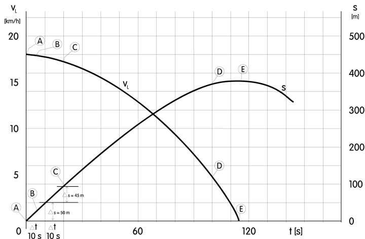
Figure 1 Stopping manoeuvre
