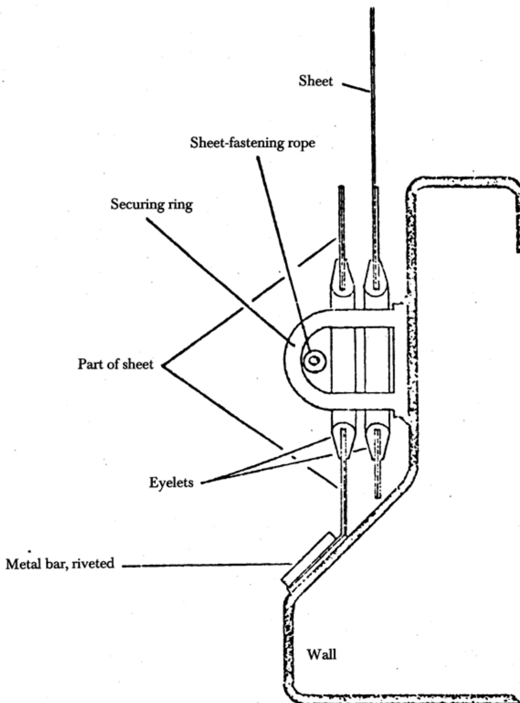
Sketch Device for fastening sheets No 4
