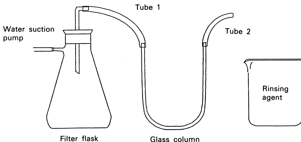
Figure 3: Arrangement for rinsing
