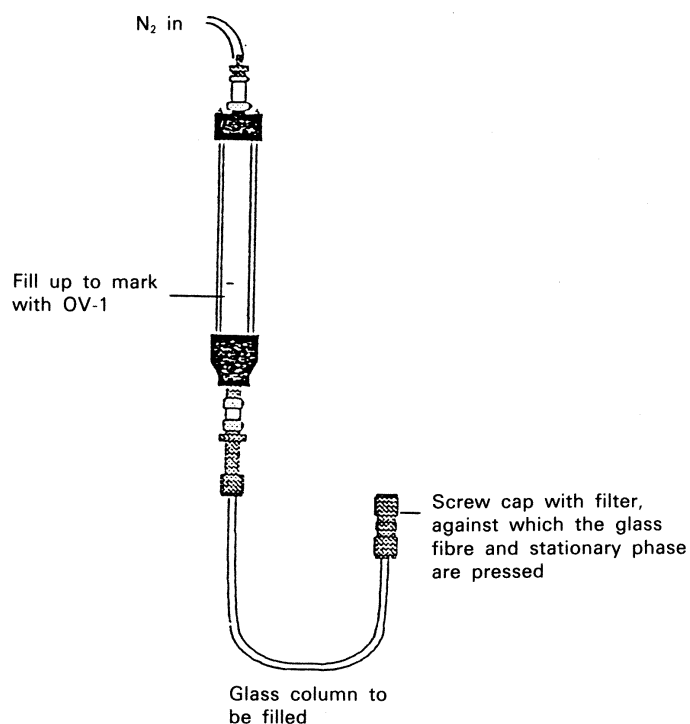
Figure 1: Filling of the column
