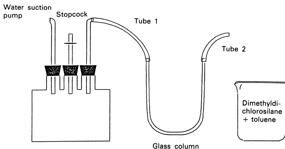
Figure 2: Arrangement for silanisation
