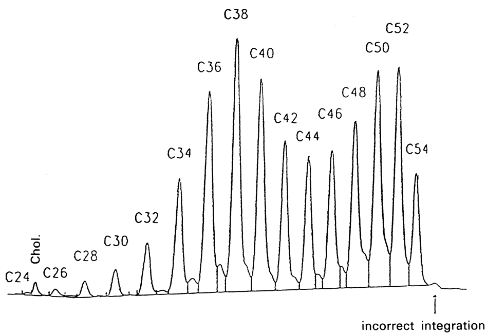
Figure 6: Wrongly integrated chromatogram of milk fat
