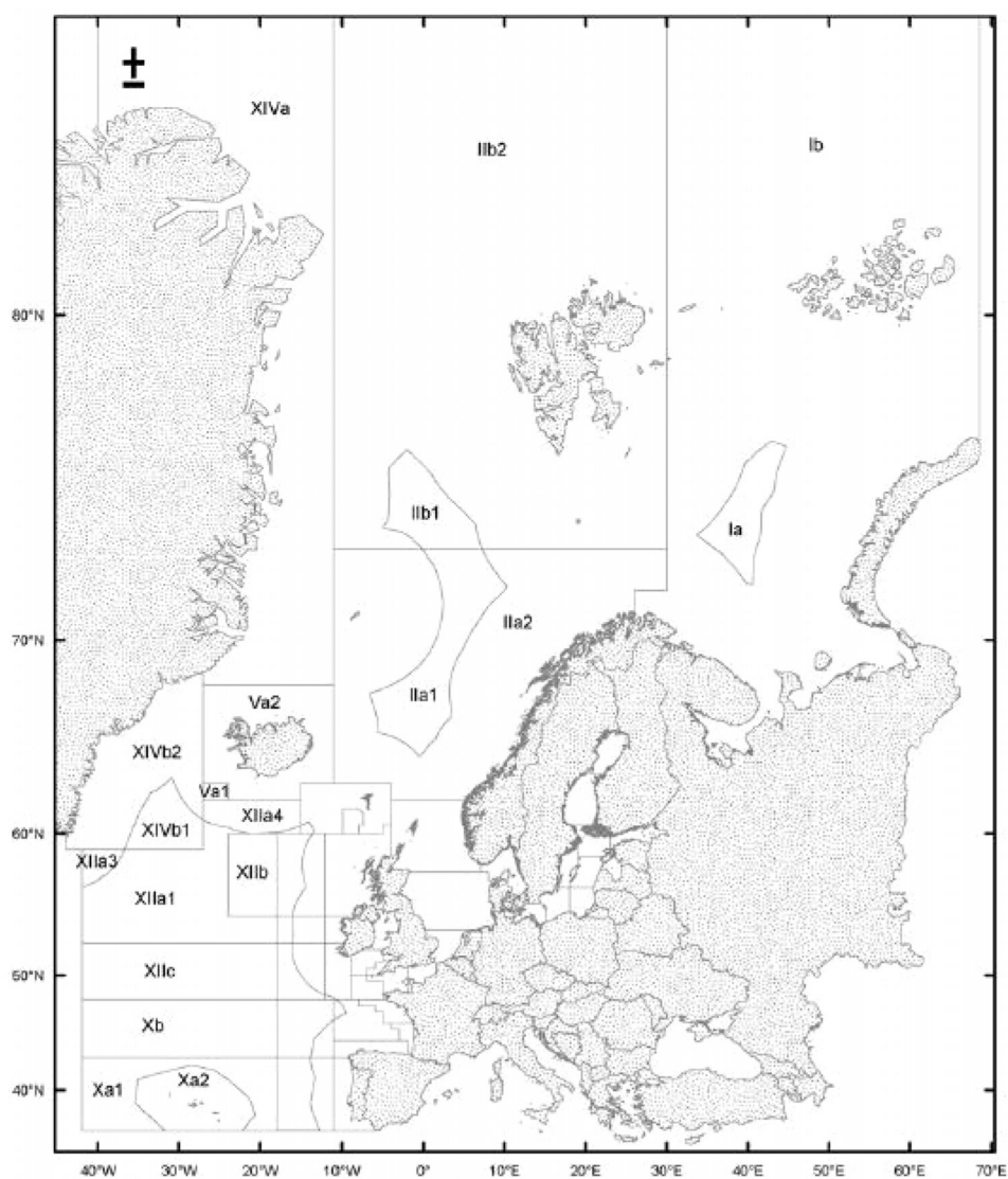
Statistical fishing regions of the north-east Atlantic
