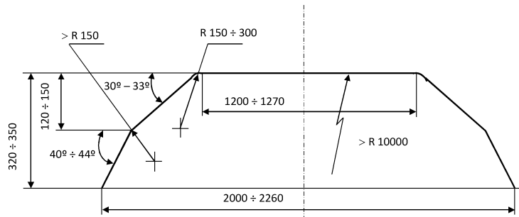
Fig. Configuration and dimensions of contact skates
