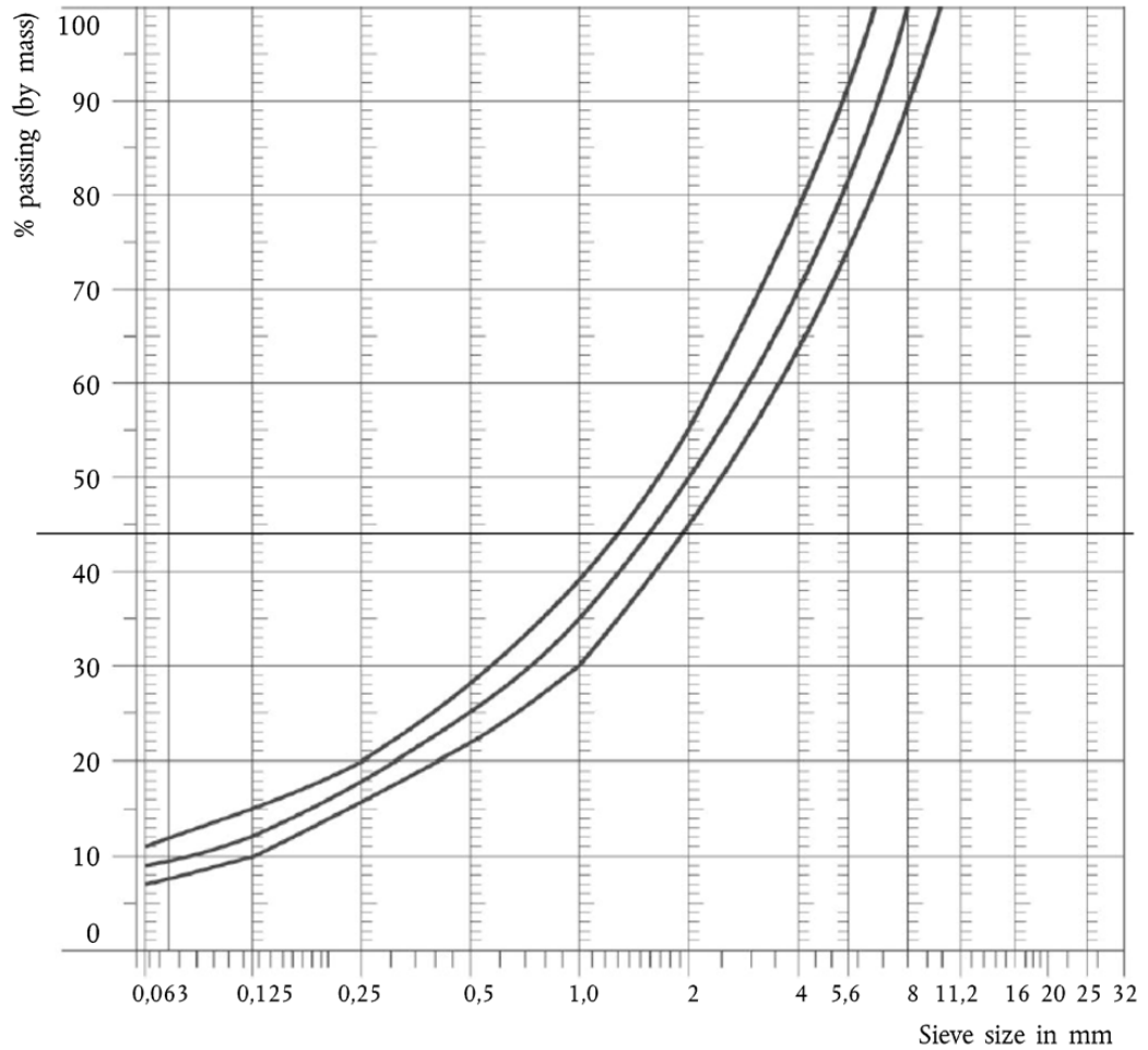
Grading curve of the aggregate in the asphaltic mix, with tolerances
