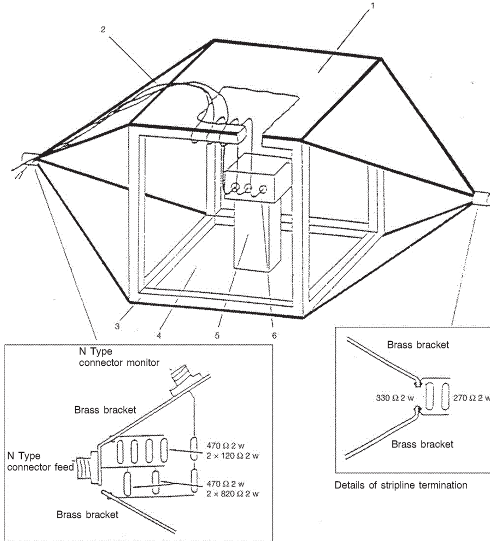
Details of stripline feed
