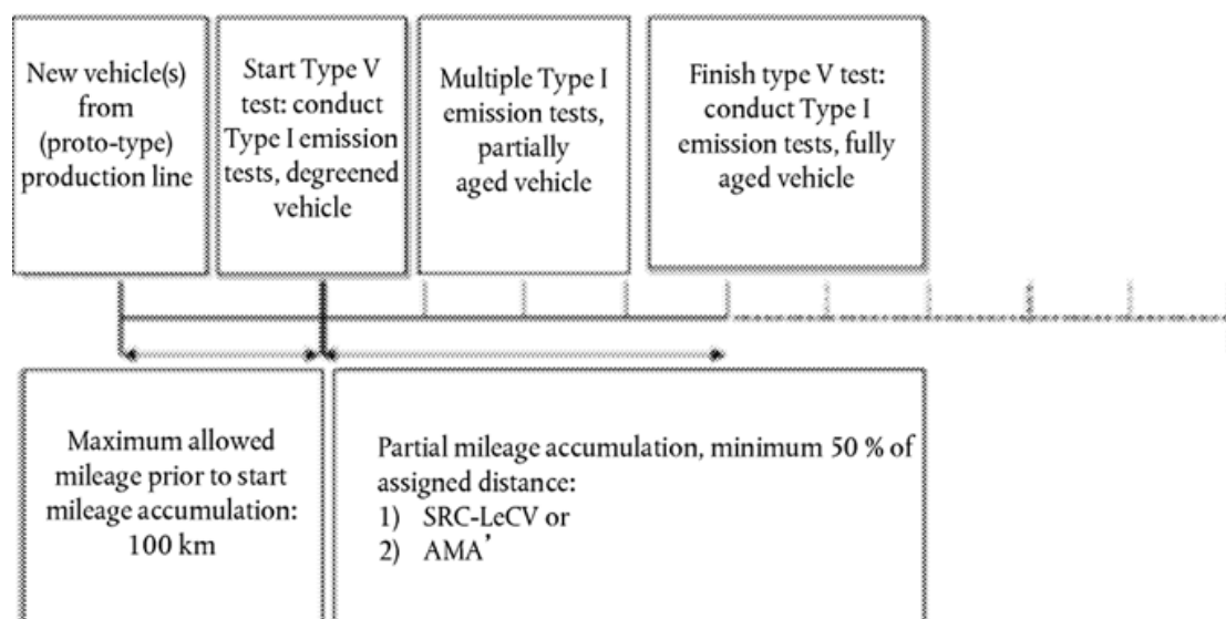
Figure 5-2 Test type V — accelerated durability test procedure with partial distance accumulation
