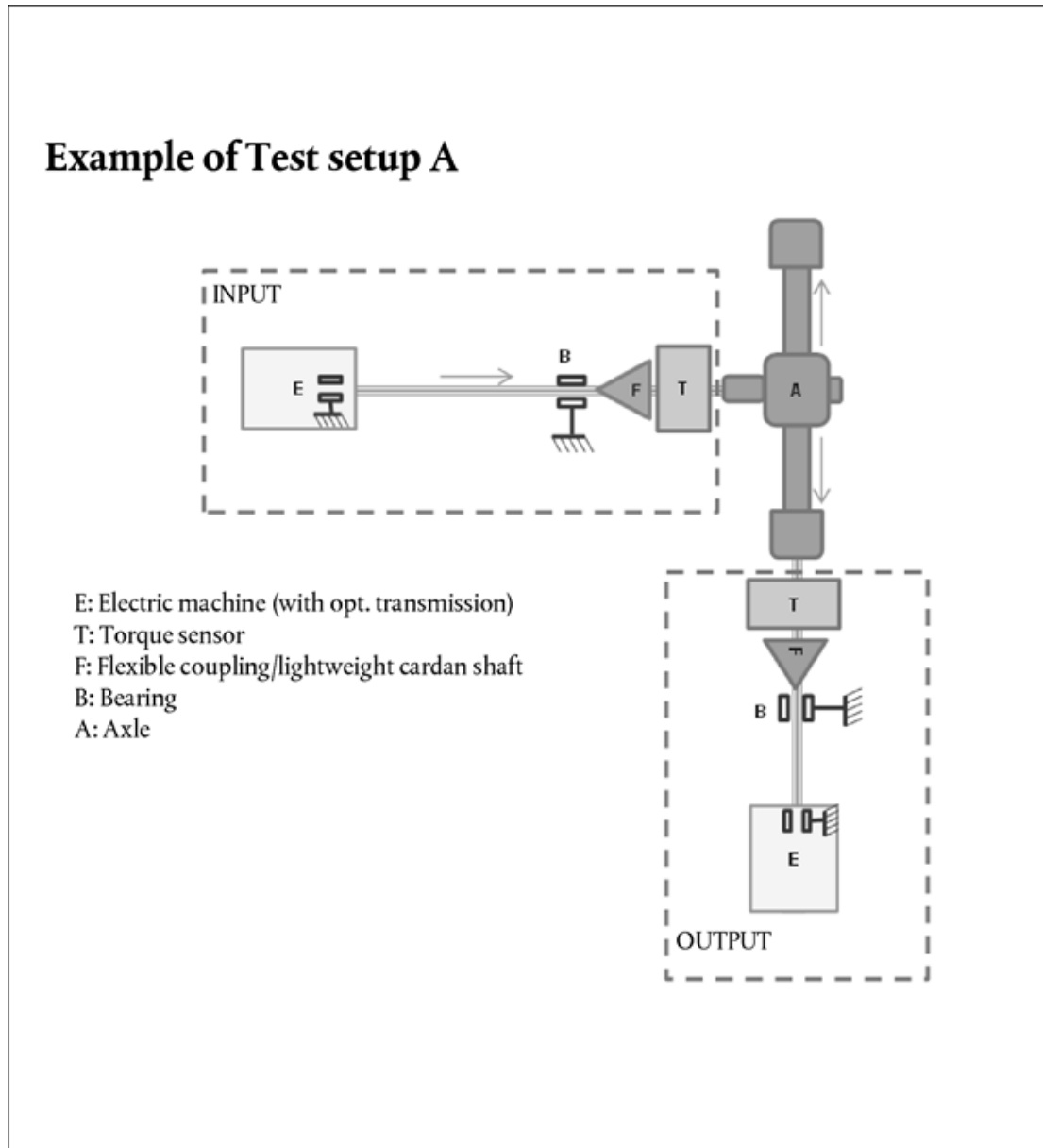
Figure 1 Example of Test set-up ‘Type A’ U.K.
