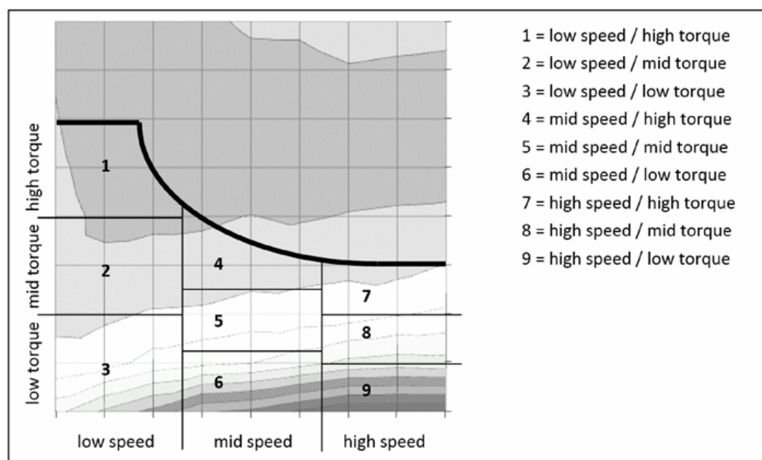
F1 Figure 2 Speed and torque range for conformity of the certified CO 2 emissions and fuel consumption related properties testing U.K.
