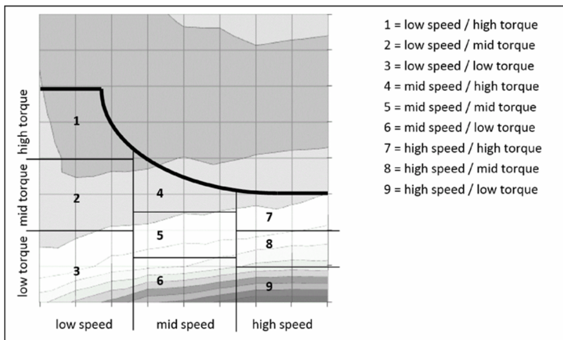
Figure 2 Speed and torque range for conformity of the certified CO 2 emissions and fuel consumption related properties testing
