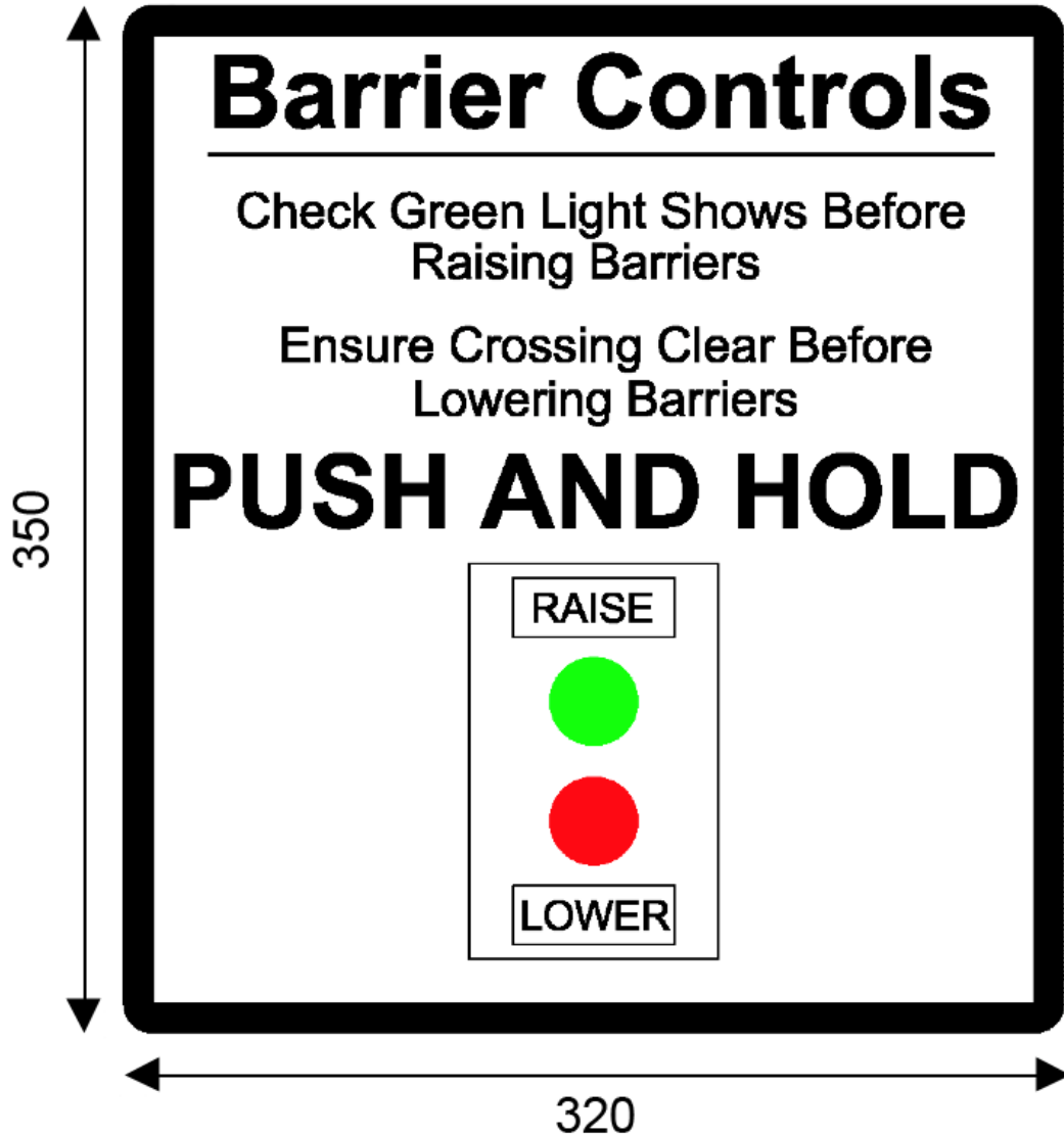
Black lettering and border on white background Instructions for Miniature Stop Light with barriers Entry Raise and Exit Lower Plungers Diagram 99
