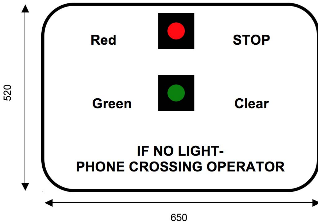
Black lettering and border on white background Sign for use with miniature stop lights at a crossing with a telephone Diagram 107
