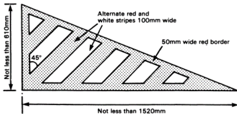
DIAGRAM OF SIDE MARKER SURFACE
