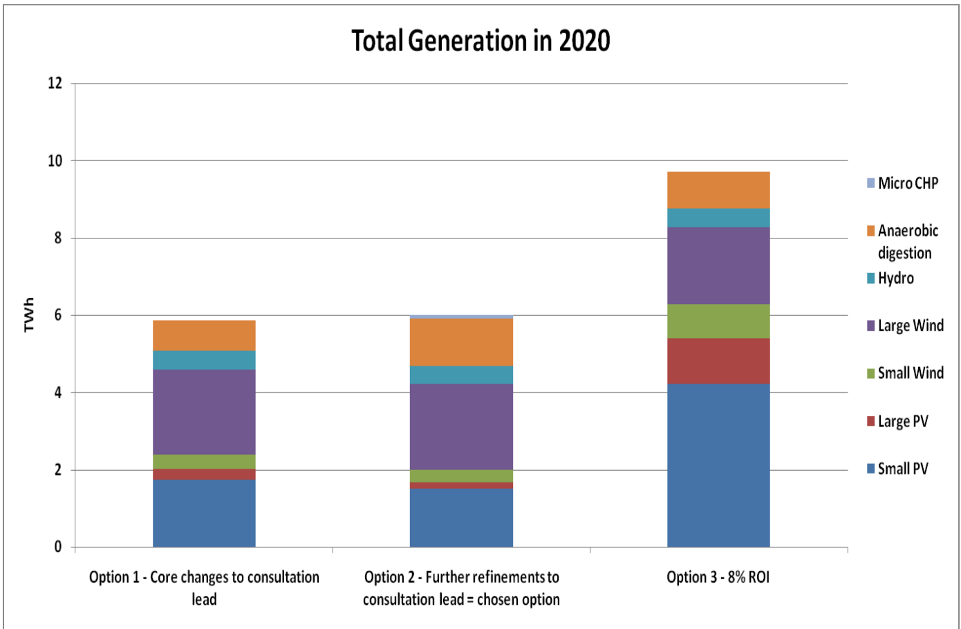
Figure 1 – Technology mix under different scenarios
