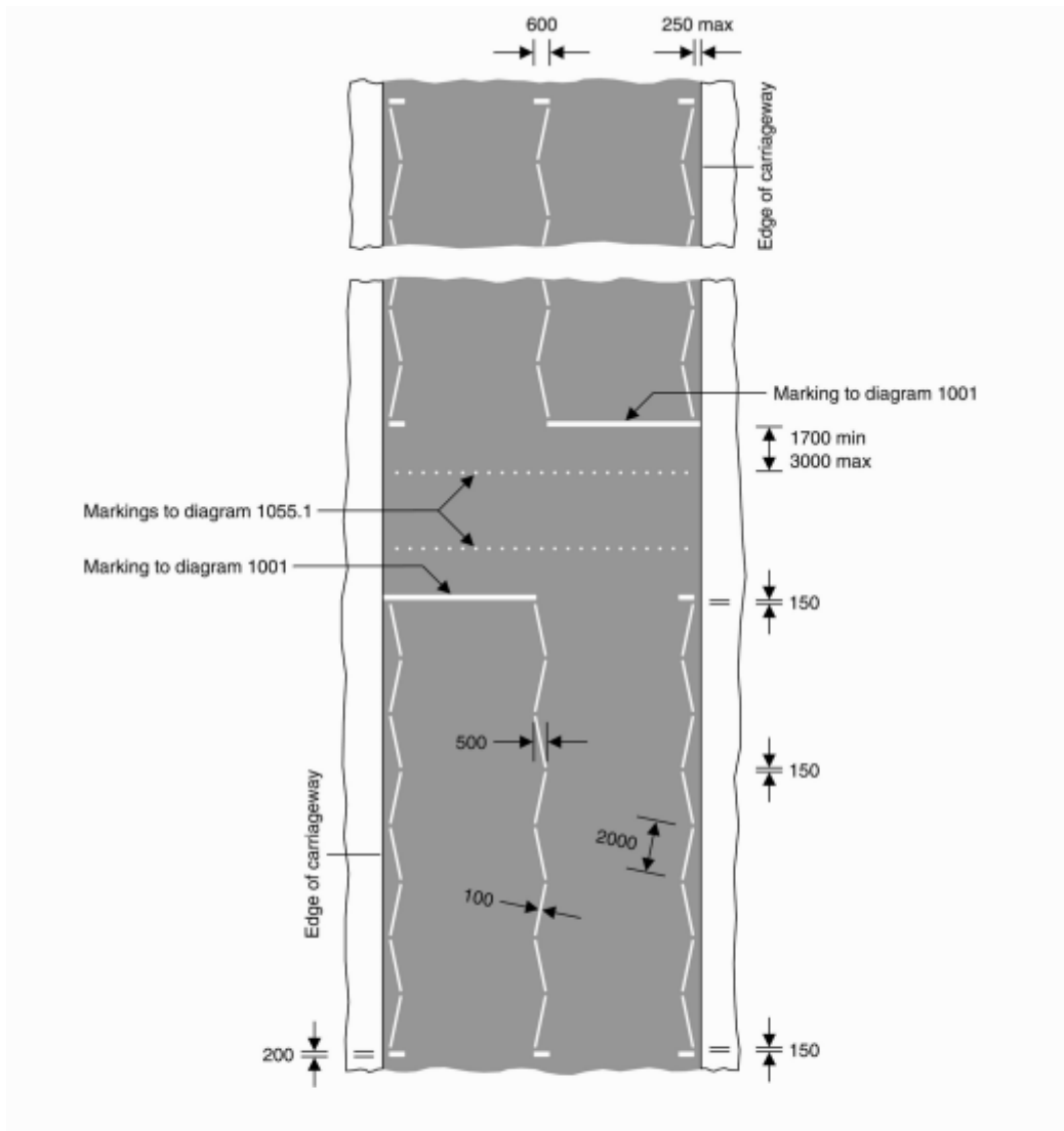
1001.3 Zig-zag lines to indicate the requirements of regulations 27 and 28 at a signal-controlled crossing facility or portable signal-controlled pedestrian facility (Shown in combination with diagrams 1001 and 1055.1)
